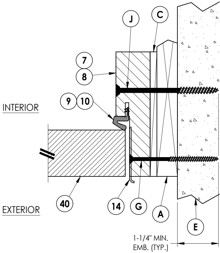
3 HORIZONTAL CROSS SECTION Shown w/ 1X sub-buck
