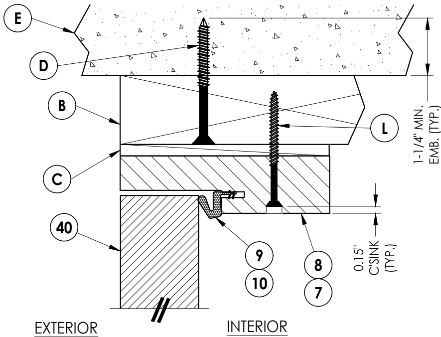
1 4 VERTICAL CROSS SECTION Outswing shown - inswing also approved
