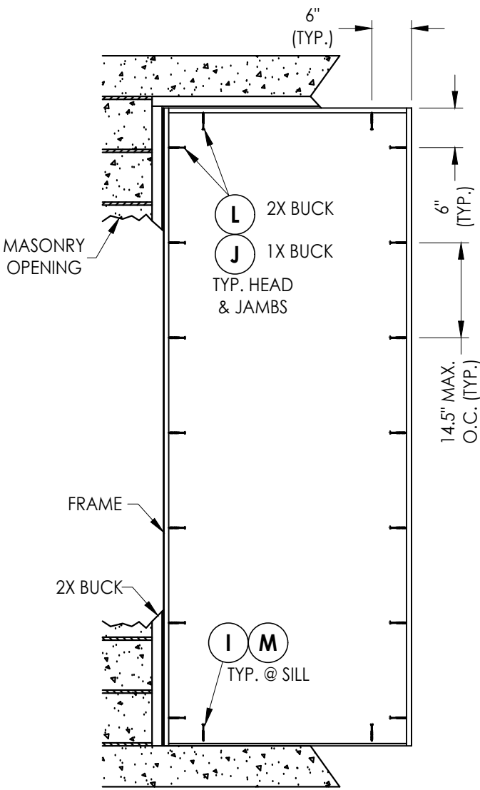
FRAME ANCHORING
