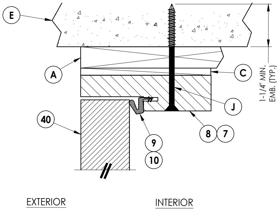
2 4 VERTICAL CROSS SECTION Shown w/ 1X sub-buck
