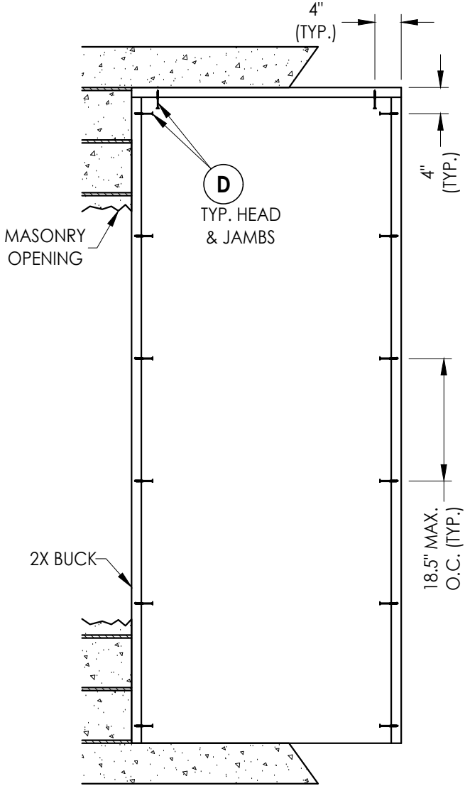
BUCK ANCHORING
